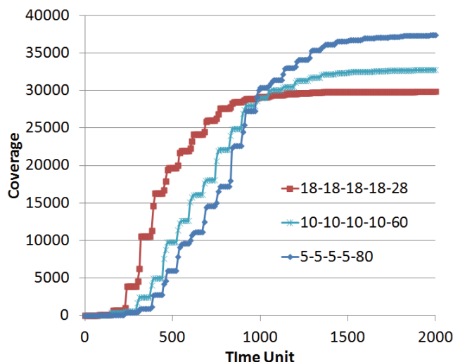
Figure 4. Propagation process with different channel preferences
