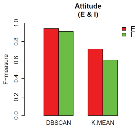
Figure 3. Performance of predicting user attitude (E: Extraversion and I: Introversion) in MBTI (Myer-Briggs Type Indicator). SVM (Support Vector Machine) is used as a classifier and each location clustering technique is used to extract classification features.
