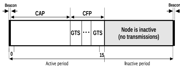
Fig. 1: Superframe structure
