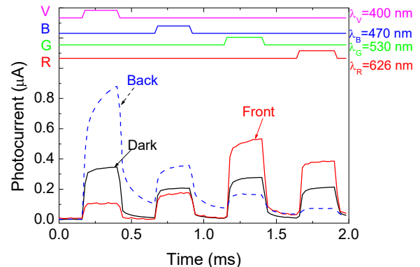
Figure 5. Transient photocurrent without (Dark) and under front (Front) and back (Back) 390 nm irradiation.
