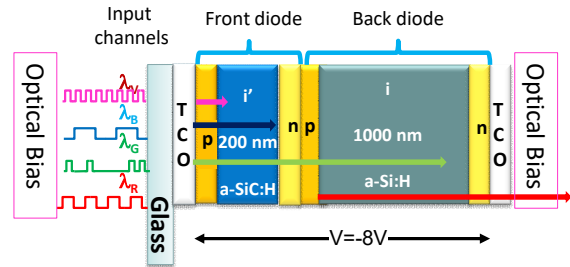
Figure 4. Double pin configuration and device operation.
