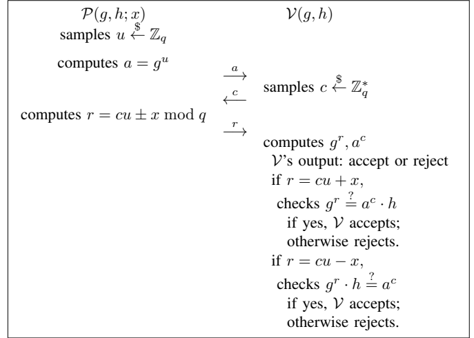
Figure 2. Protocol 2- Modified Schnorr Protocol for relation R_{ID} .
