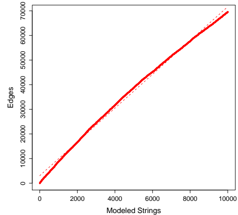
(a) Random Strings - Edges
