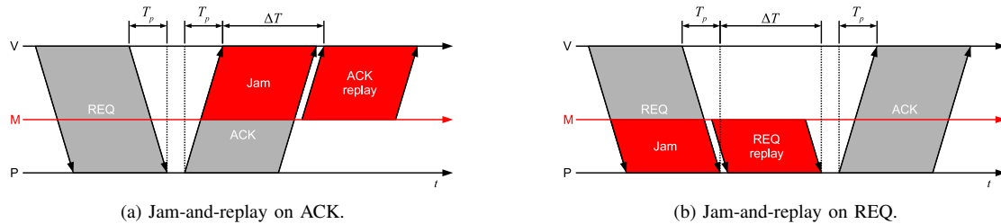
Figure 2. Jam-and-replay attack.
