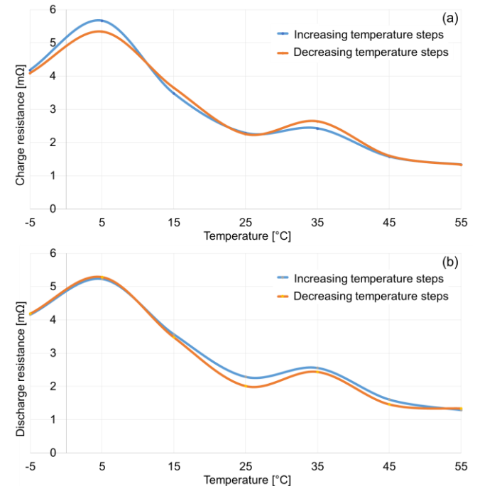
Figure 8. Battery charge and discharge series resistance at rising and falling temperatures
