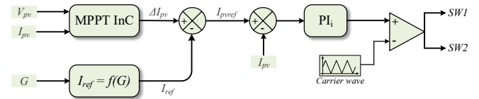
Figure 2. Strategy MPPT Control.
