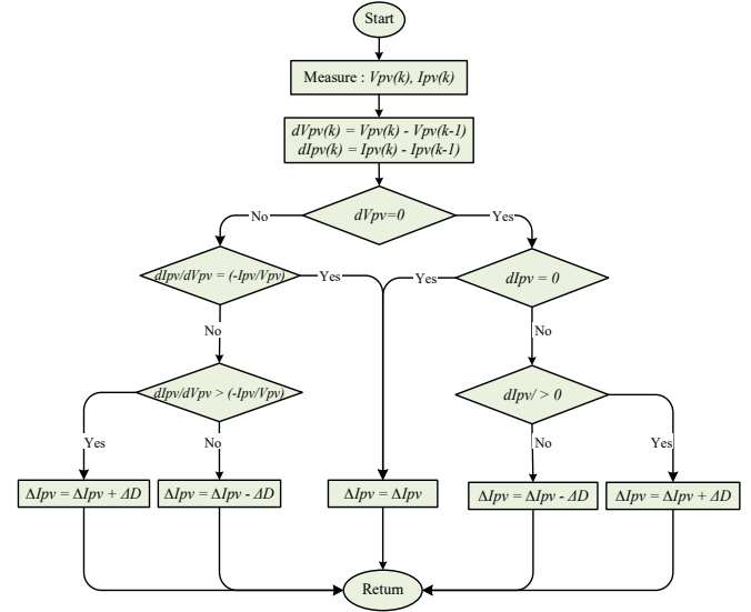
Figure 3. MPPT InC.
