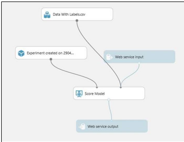
Figure 6. Azure Data Flow for Prediction Mode.
