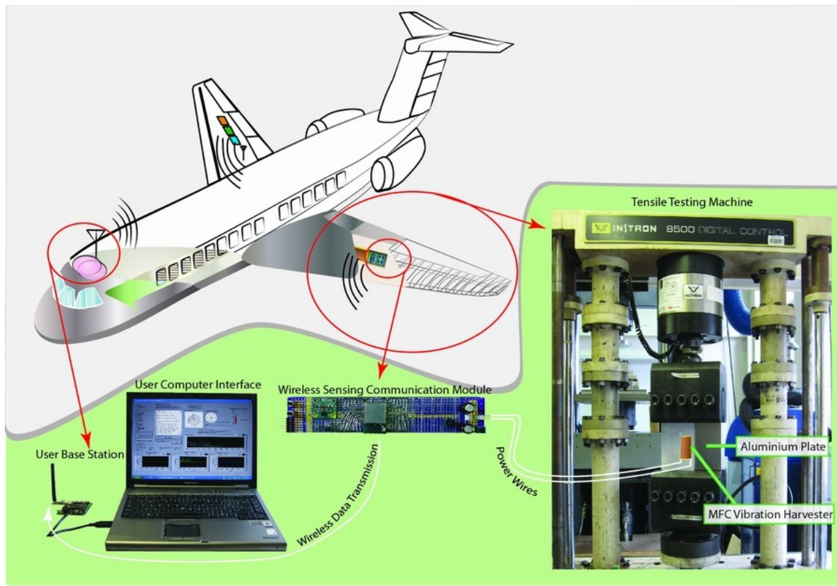
Figure 3. Structural Health Monitoring: application and laboratory testing set-up.
