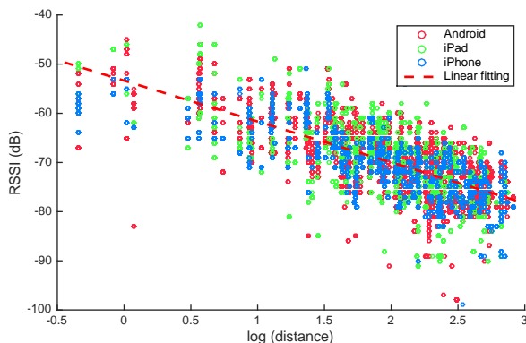
Figure 4. Plots of RSSI vs. log distance color coded by devices. A linear regression line is fitted on the data: \text{RSSI} = -8.31 \cdot \log(d) - 53.4 .
