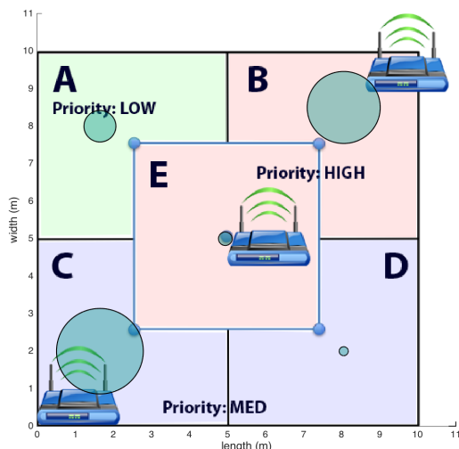
Figure 1. Map of the toy example showing the access points locations and fingerprints allocations (radius of the green circle) determined by APEC Exhaust (also APEC Greedy since they agree).
