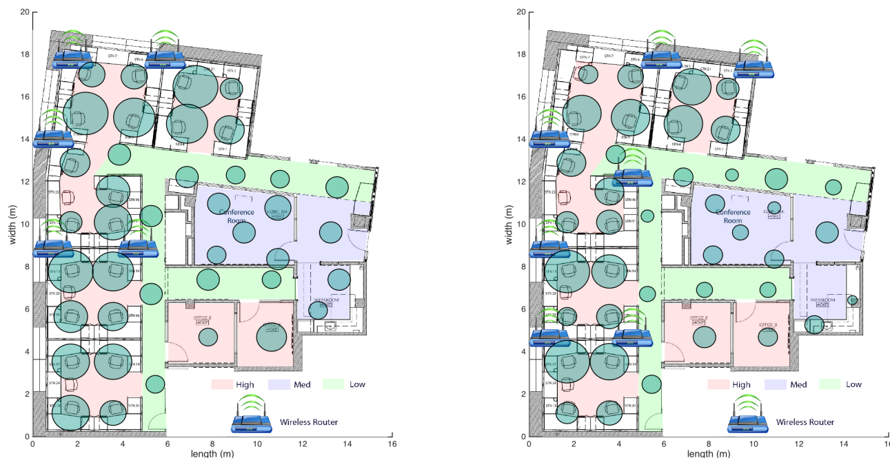
Figure 7. Visualization of IPS configuration in CREST for experiment A (left) and B (right), where 5 or 7 access points are deployed according to APEC Greedy. Location priority map is color coded as illustrated in the legend. Location frequency map is not shown, which is HIGH for cubicles, MED for shared spaces, and LOW for corridors. The radius of the green circle indicates the number of fingerprints at the spot.
