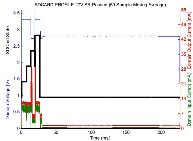
Figure 13: A Micro-SD Card Cache Miss and a Cache Hit
