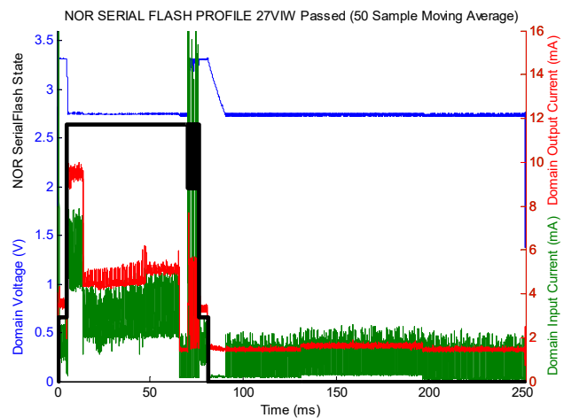
Figure 11: NOR Serial Flash Write-Cycle using IODVS and PACER-T
