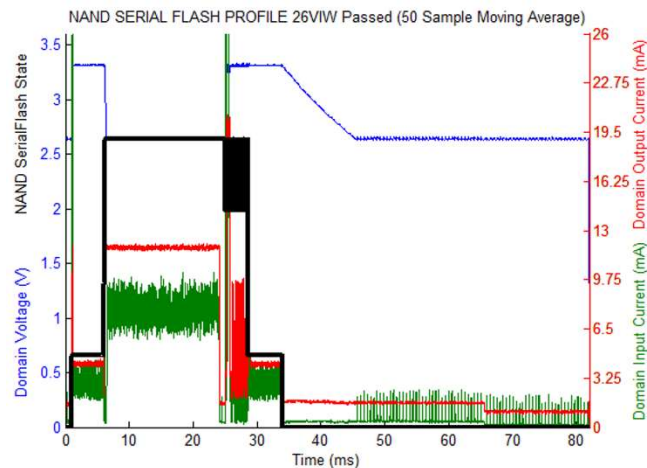
Figure 12: NAND Serial Flash Write Cycle Using IODVS and PACER-T
