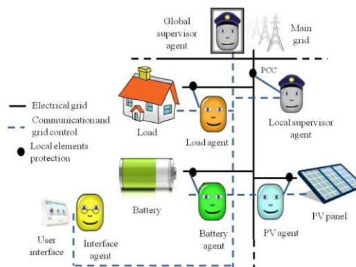
Figure 2. MAS for the proposed Microgrid management approach
