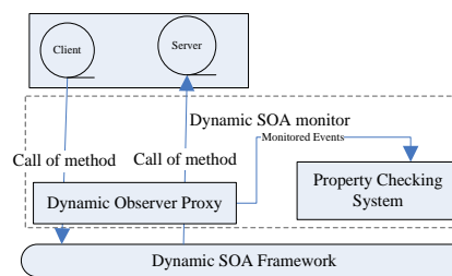
Figure 2. Monitor Abstract Architecture
