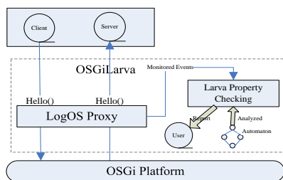
Figure 3. OSGiLarva Implementation
