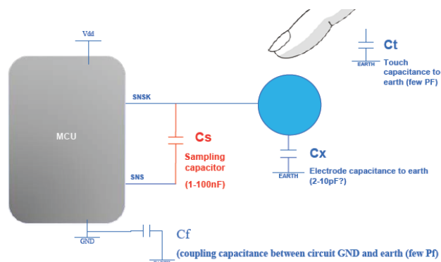
Figure 1. Self Capacitance Equivalent Circuit, [1]
