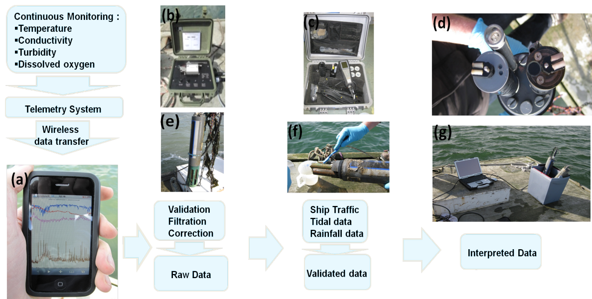
Fig. 3: Data collection, analysis and interpretation; (a) real-time data visualisation in the field using smart phones, (b) telemetry system, (c) YSI Pro-Plus hand-held sensor used for on-site validation, (d, e) YSI 6 series sonde, (f) sensor cleaning and (g) validation procedure.
