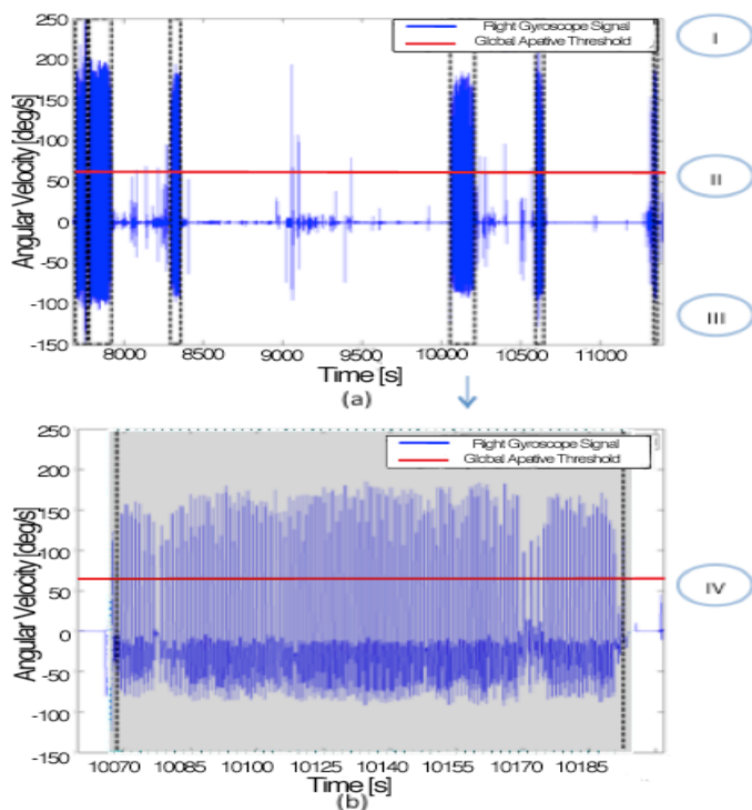
Figure 2: Example of right gyroscope signal processing through the described algorithm where the Roman Numerals in the circles refer to the steps of the algorithm. Part (a) is the gyroscope signal filtered at 3Hz. Each identified gait event is outlined by dotted rectangles. Part (b) shows the gyroscope signal for the gait event occurring between 10060 and 10210 seconds. The black dotted rectangle delineates the entire gait event identified. The shaded rectangle (slightly larger than the black dotted rectangle) shows the edges of the gait event as identified by the gait feature extraction algorithm.
