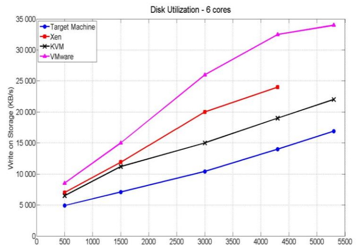
Figure 7. KVM, VMware and Xen disk utilization for 6 cores
